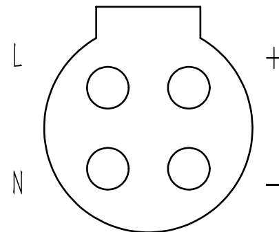
4-core male cable (+/-)
