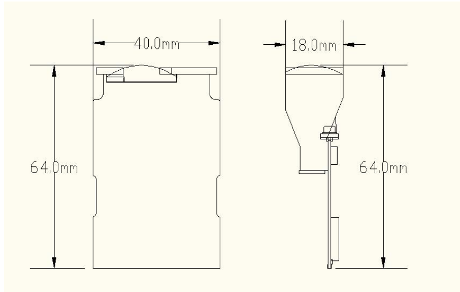
Figure 3-1 Mechanical Size
